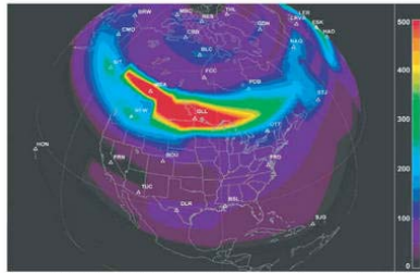
Geomagnetic field disturbance conditions, dB/dt (nT/min) over North America at time 7:45 UT on March 13, 1989 Source: Metatech Corporation, Applied Power Solutions
